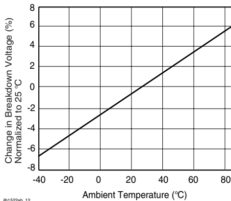
Figure 13. Switch Breakdown Voltage vs. Temperature
