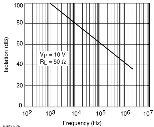
Figure 10. Output Isolation
