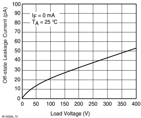
Figure 11. Leakage Current vs. Applied Voltage
